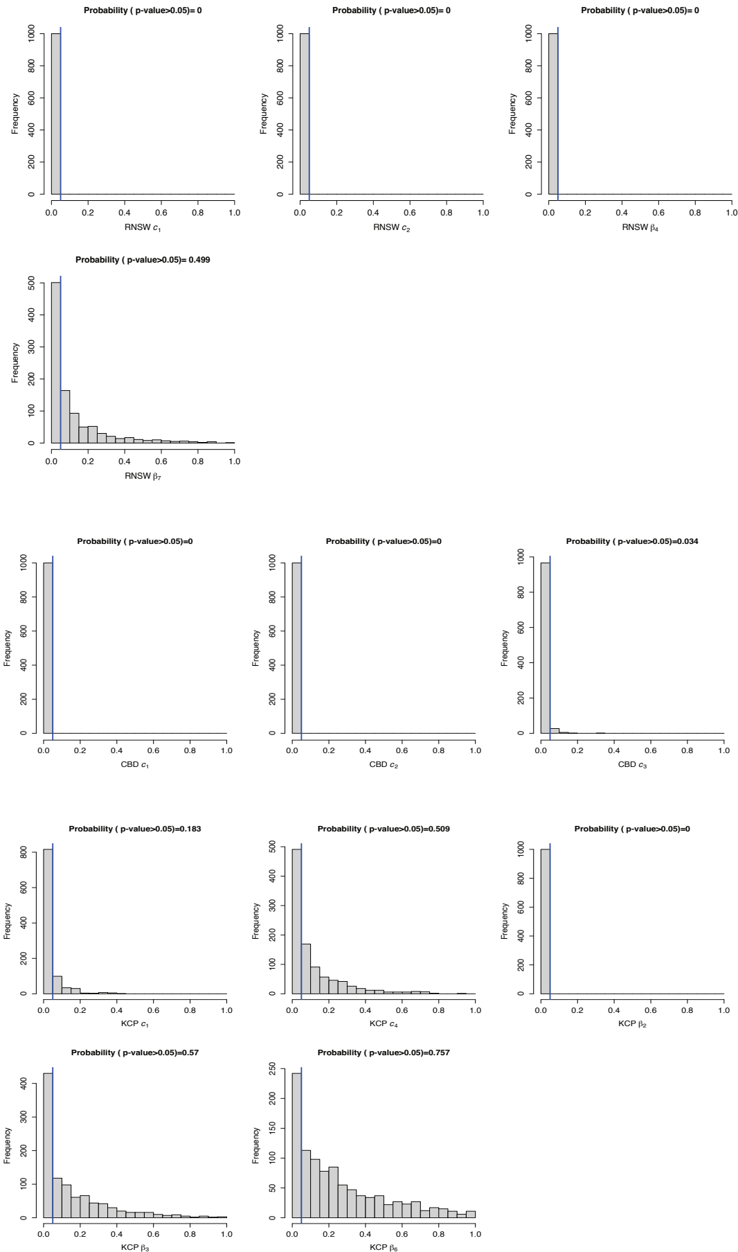
Figure A3. Reduced intervention model: Histograms of p -values for the hypothesis c_k = 0 versus c_k \neq 0 , and \beta_k = 0 versus \beta_k \neq 0 for each of the k = 1, \dots, 7/5/6 policies in RNSW (top), the CBD (middle) and KCP (bottom), over all 1,000 difference dataset replications. Vertical line indicates p=0.05 . Proportion of p -values greater than 0.05 is shown in plot title
