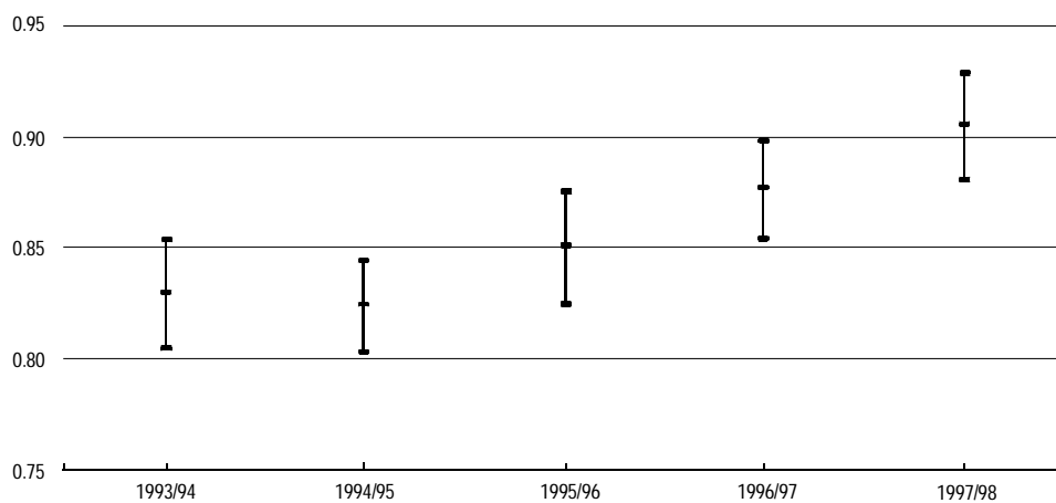
Figure 19: Annual means and 95% confidence intervals for estimates of parameter j , July 1993 to June 1998
