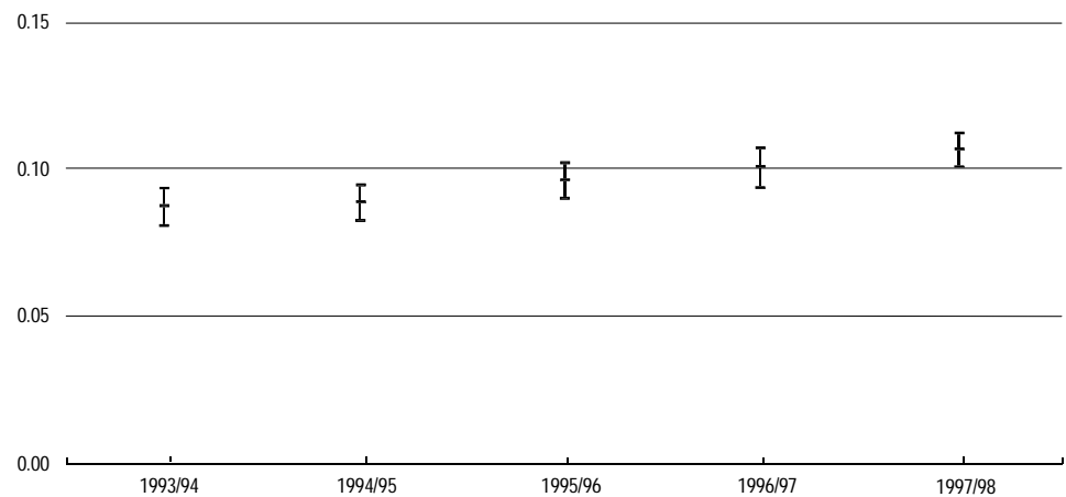
Figure 20: Annual means and 95% confidence intervals for estimates of parameter p , July 1993 to June 1998
