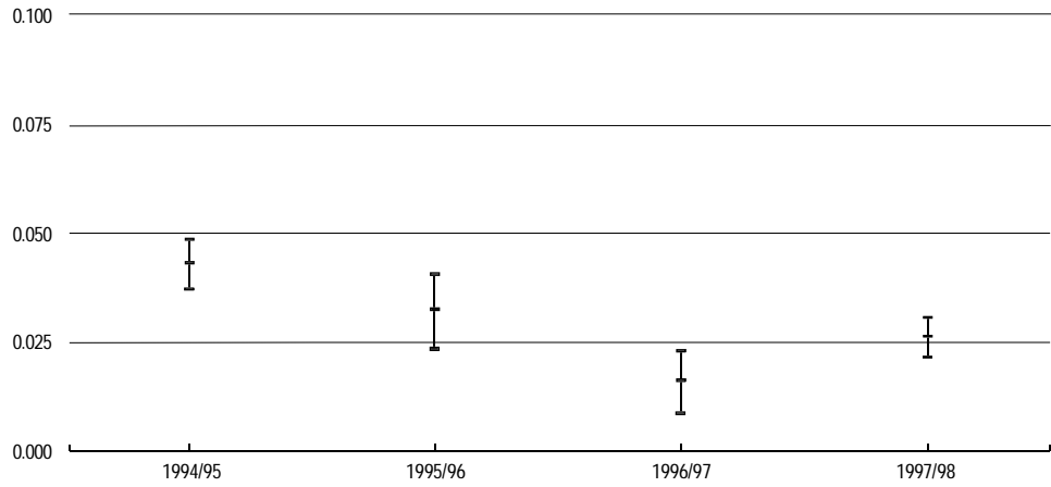
Figure 17: Annual means and 95% confidence intervals for estimates of parameter h , July 1994 to June 1998
