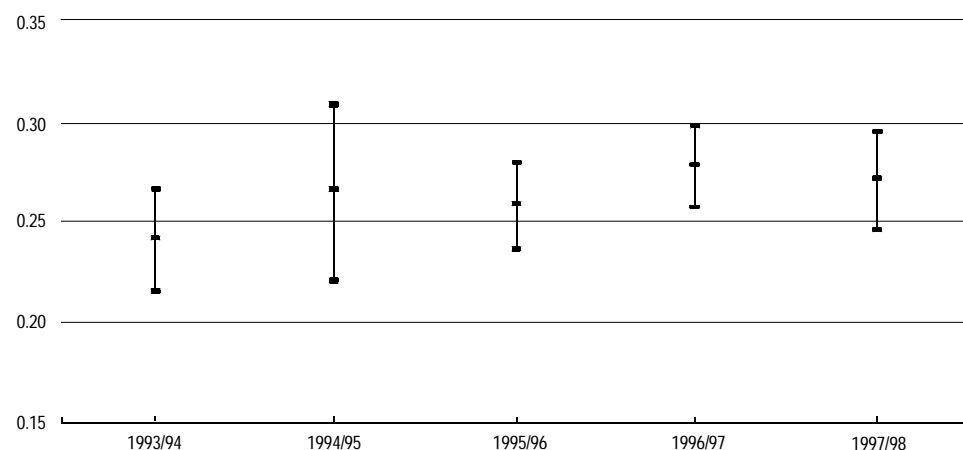
Figure 15: Annual means and 95% confidence intervals for estimates of parameter g , July 1993 to June 1998
