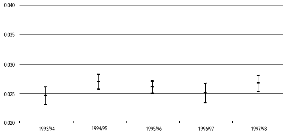
Figure 13: Annual means and 95% confidence intervals for estimates of parameter e , July 1993 to June 1998
