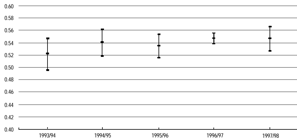
Figure 10: Annual means and 95% confidence intervals for estimates of parameter b , July 1993 to June 1998
