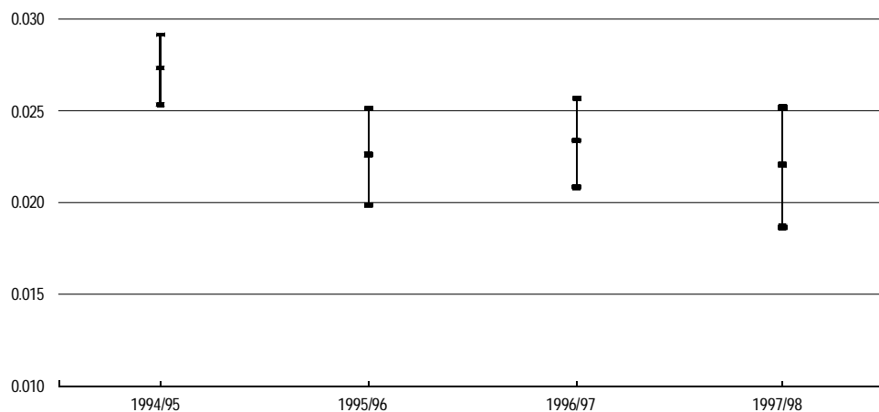
Figure 11: Annual means and 95% confidence intervals for estimates of parameter c , July 1994 to June 1998
