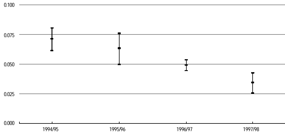
Figure 12: Annual means and 95% confidence intervals for estimates of parameter d , July 1994 to June 1998
