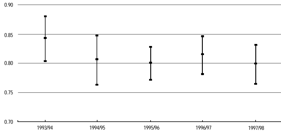
Figure 14: Annual means and 95% confidence intervals for estimates of parameter f , July 1993 to June 1998
