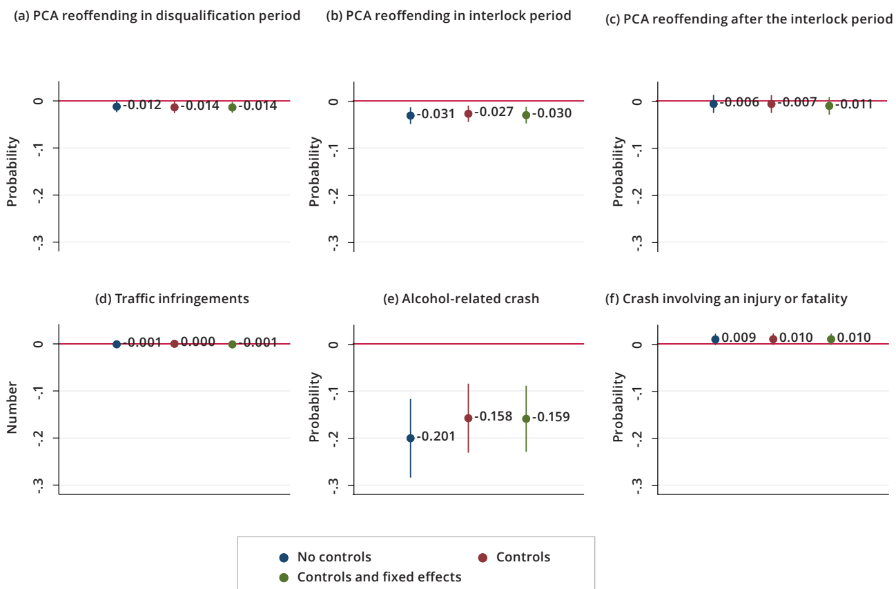
Figure A3. Sharp RD estimates between 01 February 2012 to 01 February 2015
